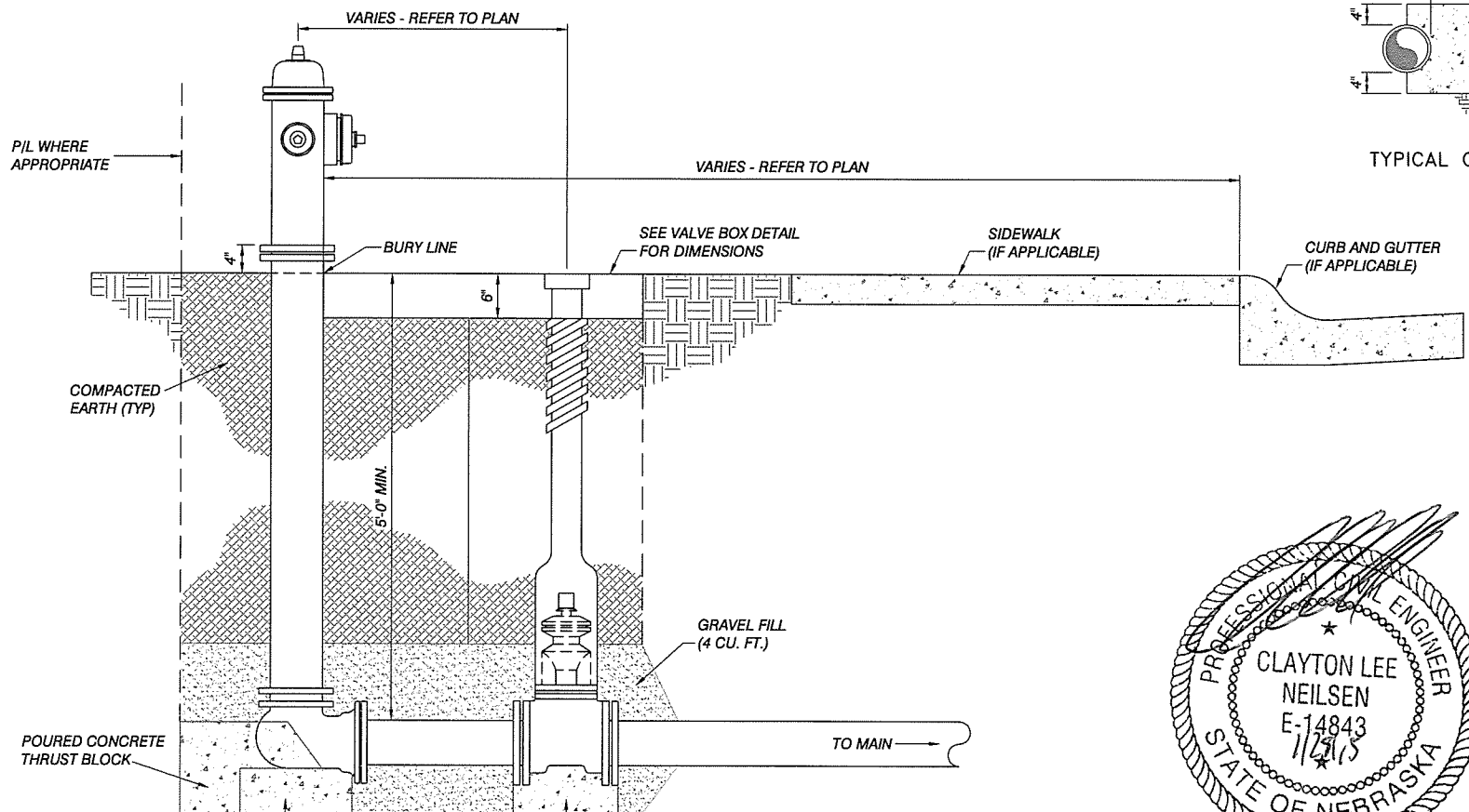
SIDE VIEW FIRE HYDRANT SETTING
