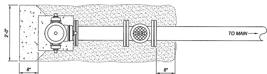
PLAN VIEW
