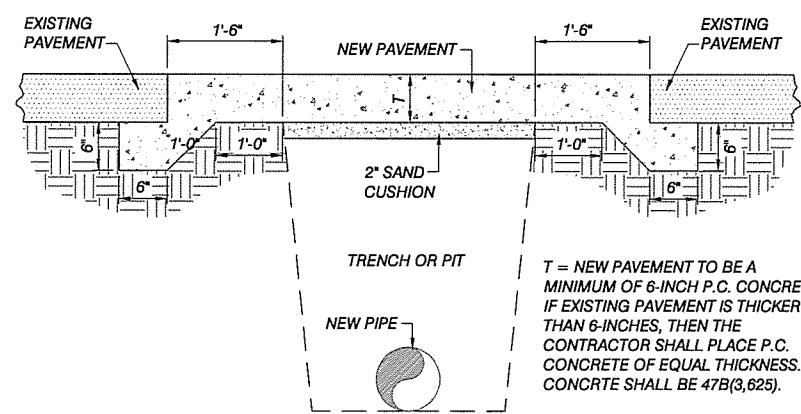
CONCRETE PAVEMENT REPLACEMENT DETAIL
