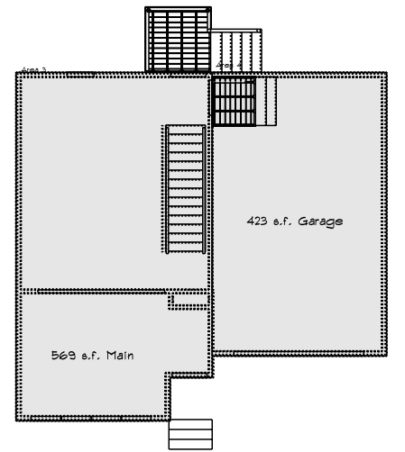
Basement SCALE: 1/16" = 1'-0"
