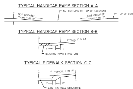
HANDICAP RAMP TYPE 3
