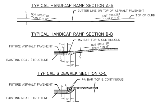
HANDICAP RAMP TYPE 4
