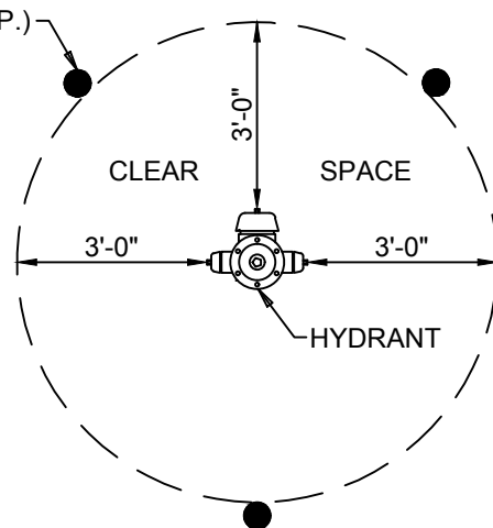
FIRE HYDRANT BOLLARD PROTECTION- TYPE B
