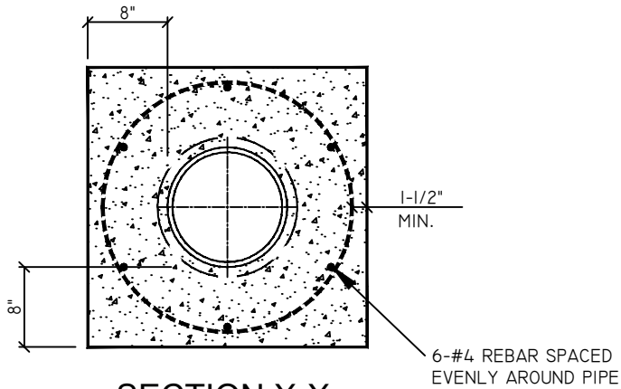
SECTION X-X
